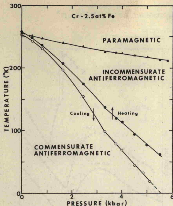
Fig. 2 The magnetic phase diagram for the 2.5% alloy. The arrows indicate the hysteresis.
