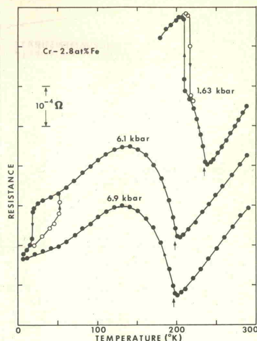
Fig. 1 Typical resistance isobars for the 2.8% alloy. The arrows indicate the location of the inflection points.
