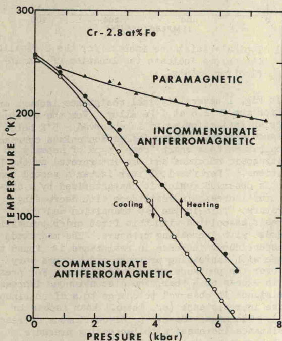
Fig. 3 The magnetic phase diagram for the 2.8% alloy. The arrows indicate the hysteresis.
